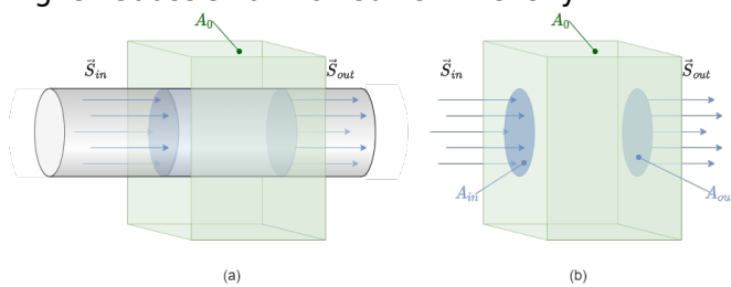
Fig. 5: Gauss's Law for Current Density
